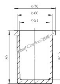
1公斤石英外套 型号: C.CC.1000A 重量: 153g 1kg ceramic shielded Model: C.CC.1000A Weight: 153g 包装 Package: 450x300x240mm (72pcs/Carton)
