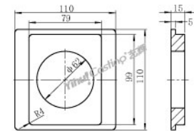
Small flange Model: C.CA.FM009 Weight: 171g
