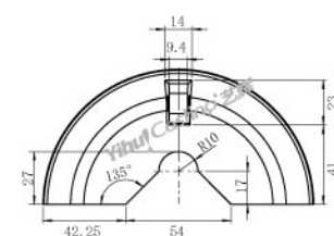
石英前盖 型号: C.CA.00008-A 重量: 136g Ceramic front cover Model: C.CA.00008-A Weight: 136g
