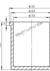
3公斤石英外套-A 型号: C.CC.3000A 重量: 324g 3kg ceramic shielded-A Model: C.CC.3000A Weight: 324g 包装 Package: 420x315x348mm (36pcs/Carton)
