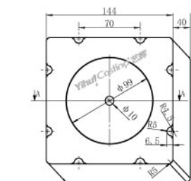
Square lid Model: C.CA.FM010 Weight: 1042g
