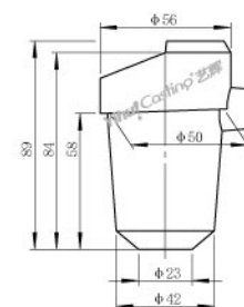
250C石英铸造坩埚 型号: C.CP.0250C 重量: 174g 250C ceramic casting crucible Model: C.CP.0250C Weight: 174g 包装 Package: 450x300x240mm (92pcs/Carton)
