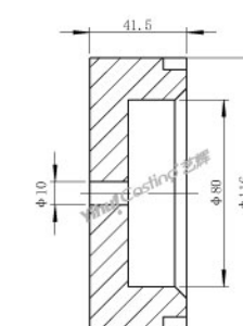
石英炉盖 型号: C.CA.FM002 重量: 511g Ceramic cover Model: C.CA.FM002 Weight: 511g 包装 Package: 420x315x348mm (69pcs/Carton)
